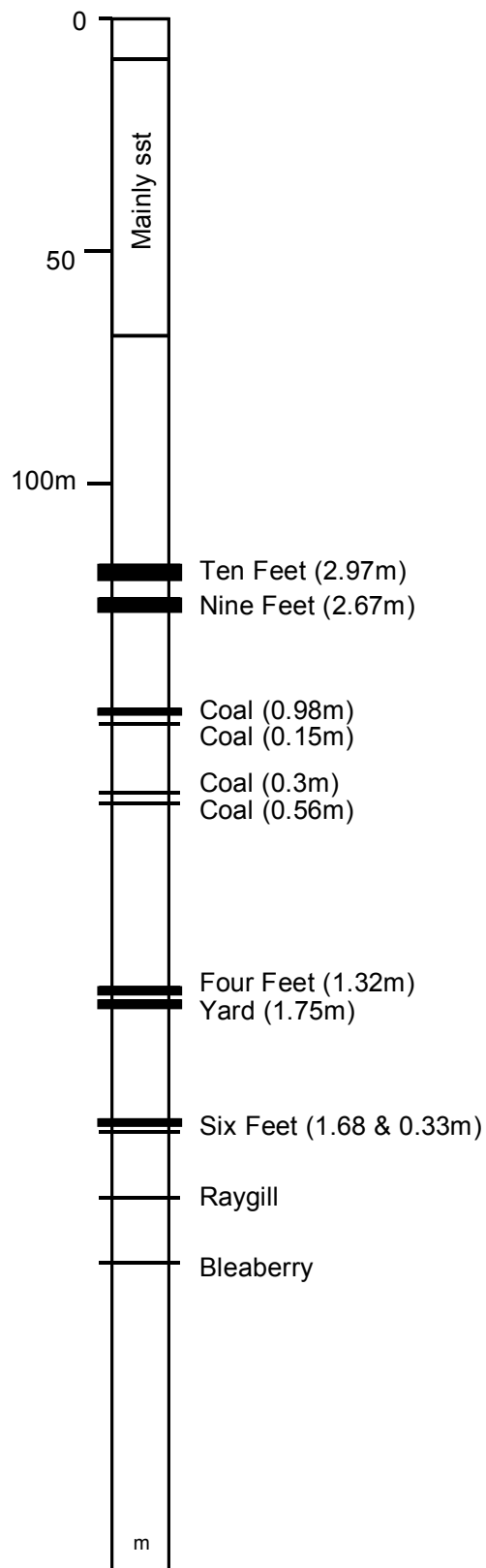
Figure 31. Stratigraphy of the main coal-bearing stratigraphic succession in the Ingleton Coalfield. Main seam names and thicknesses, where known, are labelled. m=marine band; E=Estheria band. Italicised text represent marine (or Estheria) band names.
