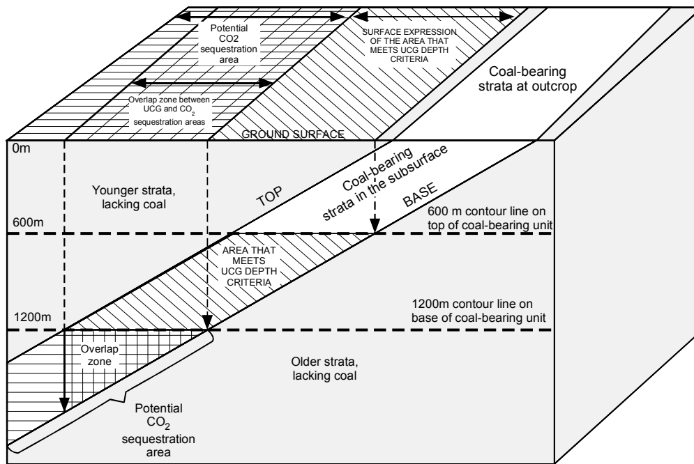
Figure 4. Block diagram of a dipping coal-bearing succession to show how the criteria for UCG and CO 2 sequestration are applied.
