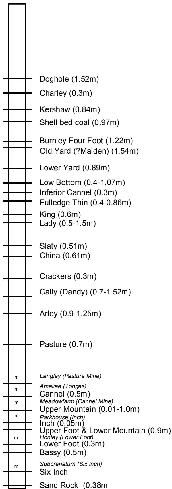
Figure 25. Stratigraphy of the main coal-bearing stratigraphic succession in the Burnley Coalfield. Main seam names and thicknesses, where known, are labelled. m=marine band; E=Estheria band. Italicised text represent marine (or Estheria) band names.
