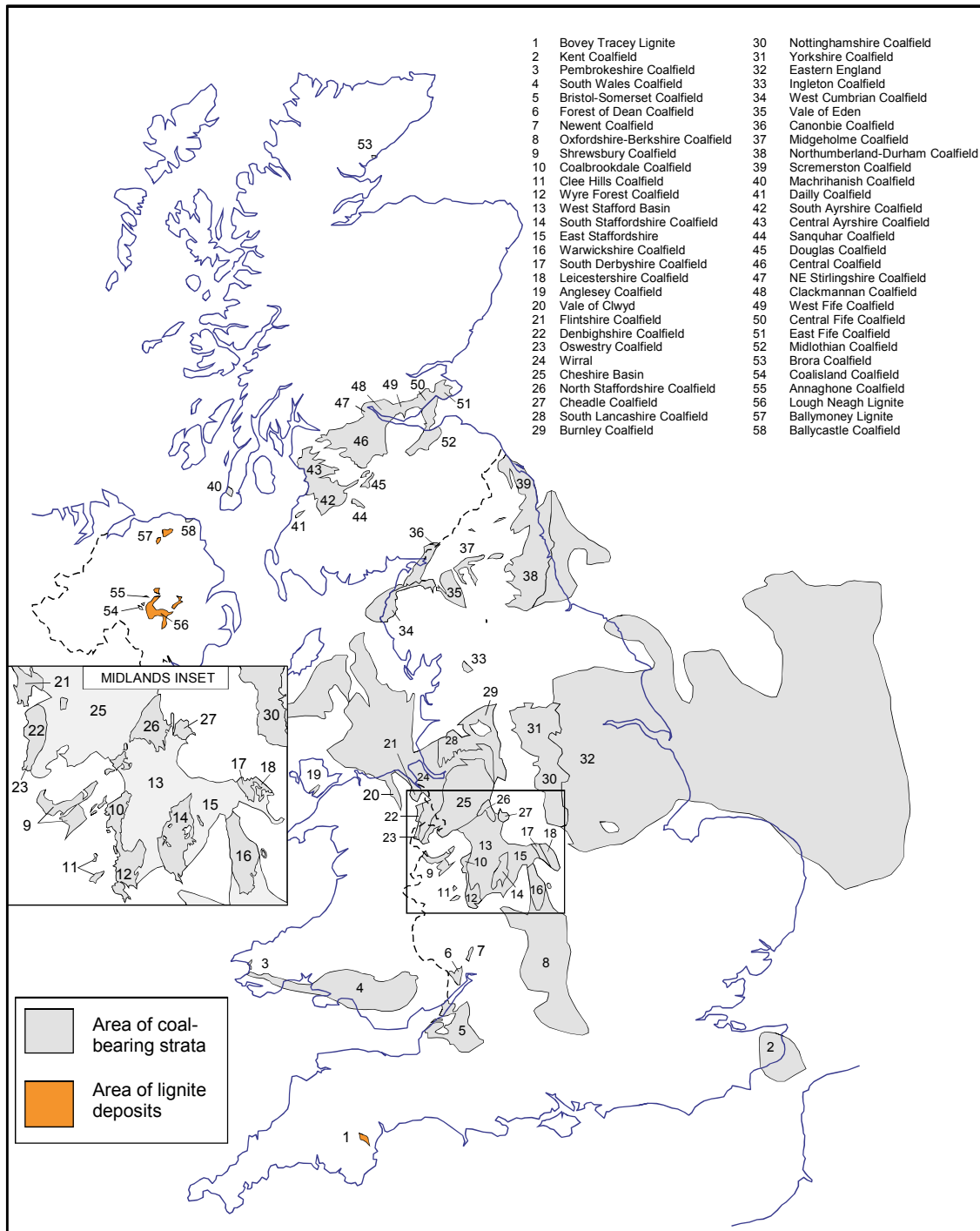
Figure 2. Map of the UK to show the location of the main coal and lignite fields studied.
