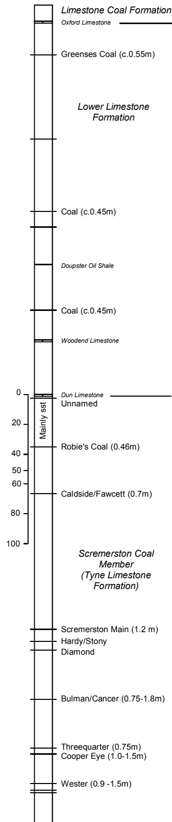
Figure 36. Stratigraphy of the main coal-bearing stratigraphic succession in the Scremerston Coalfield. Main seam names and thicknesses, where known, are labelled. m=marine band; E=Estheria band. Italicised text represent marine (or Estheria) band names.
