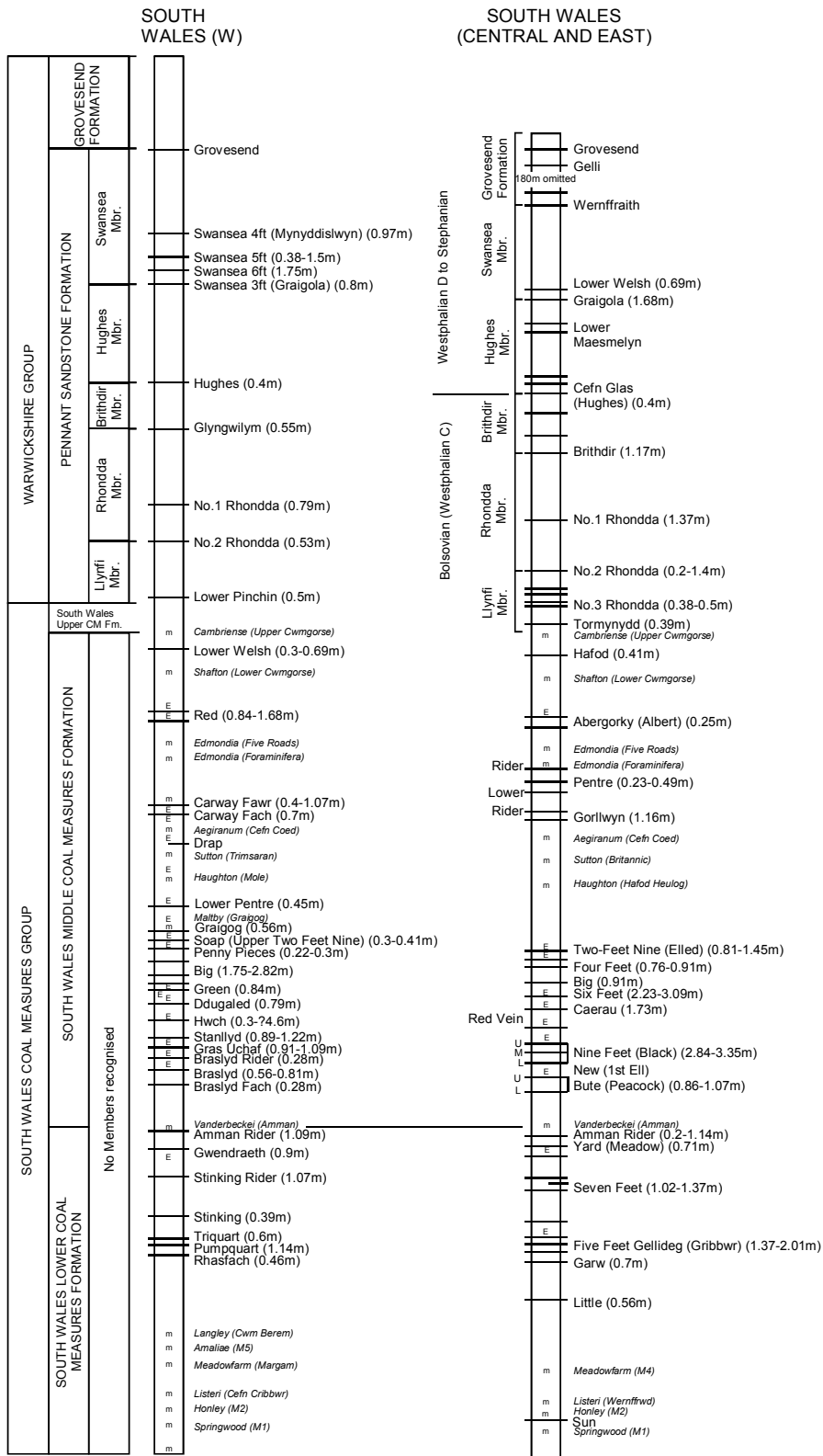
Figure 10. Stratigraphy of the main coal-bearing stratigraphic succession in the South Wales Coalfield. Main seam names and thickness, where known, are labelled. m=marine band; E=Estheria band. Italicised text represent marine (or Estheria) band names.
