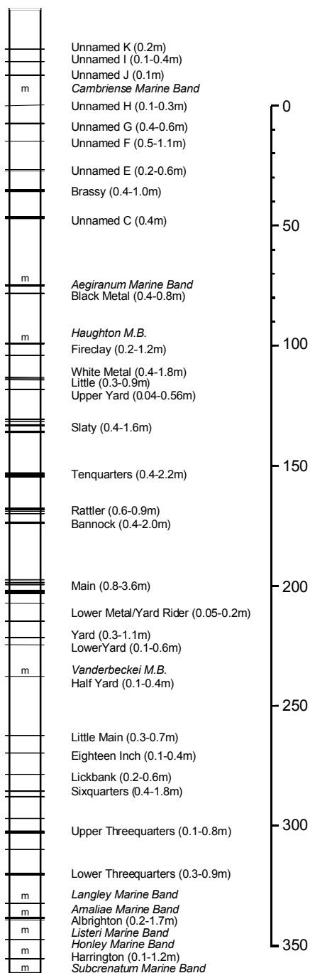
Figure 32. Stratigraphy of the main coal-bearing stratigraphic succession in the West Cumbrian Coalfield. Main seam names and thicknesses, where known, are labelled. m=marine band; E=Estheria band. Italicised text represent marine (or Estheria) band names.
