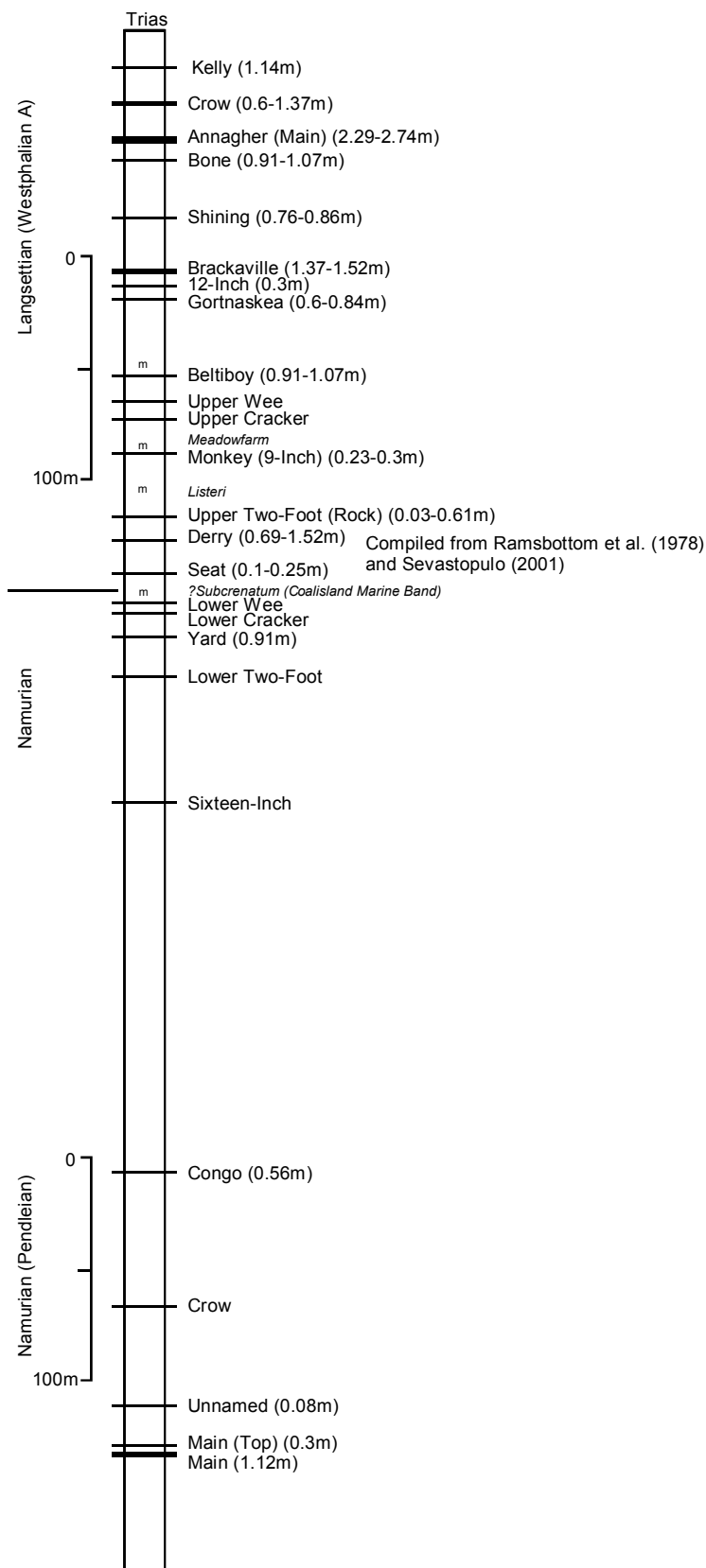
Figure 41. Stratigraphy of the main coal-bearing stratigraphic succession in the Coalisland Coalfield, Northern Ireland. Main seam names and thicknesses, where known, are labelled. m=marine band; E=Estheria band. Italicised text represent marine (or Estheria) band names.
