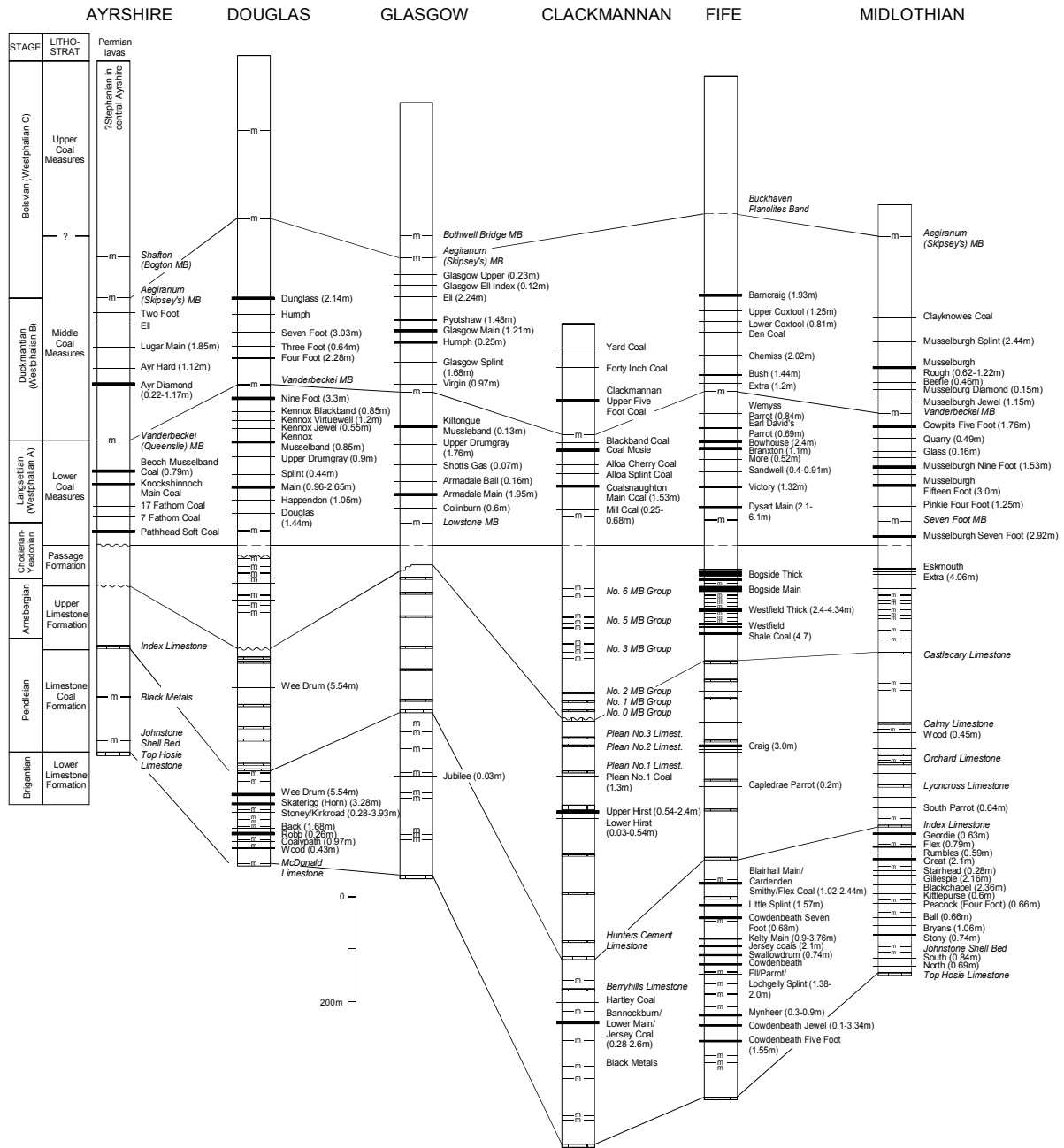
Figure 38. Stratigraphy of the main coal-bearing stratigraphic successions in the Midland Valley of Scotland. Main seam names and thicknesses, where known, are labelled. m=marine band; E=Estheria band. Italicised text represent marine (or Estheria) band names.
