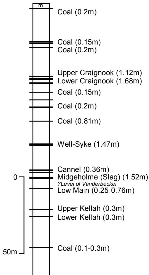
Figure 34. Stratigraphy of the main coal-bearing stratigraphic succession in the Midgeholme Coalfield. Main seam names and thicknesses, where known, are labelled. m=marine band; E=Estheria band. Italicised text represent marine (or Estheria) band names.
