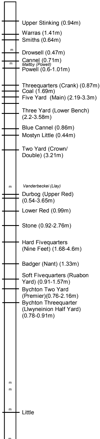
Figure 24. Stratigraphy of the main coal-bearing stratigraphic succession in the North Wales Coalfield. Main seam names and thicknesses, where known, are labelled. m=marine band; E=Estheria band. Italicised text represent marine (or Estheria) band names.
