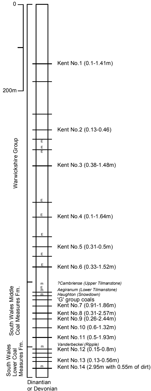
Figure 8. Stratigraphy of the main coal-bearing stratigraphic succession in the Kent Coalfield. Main seam names and thicknesses, where known, are labelled. m=marine band; E=Estheria band. Italicised text represent marine (or Estheria) band names.
