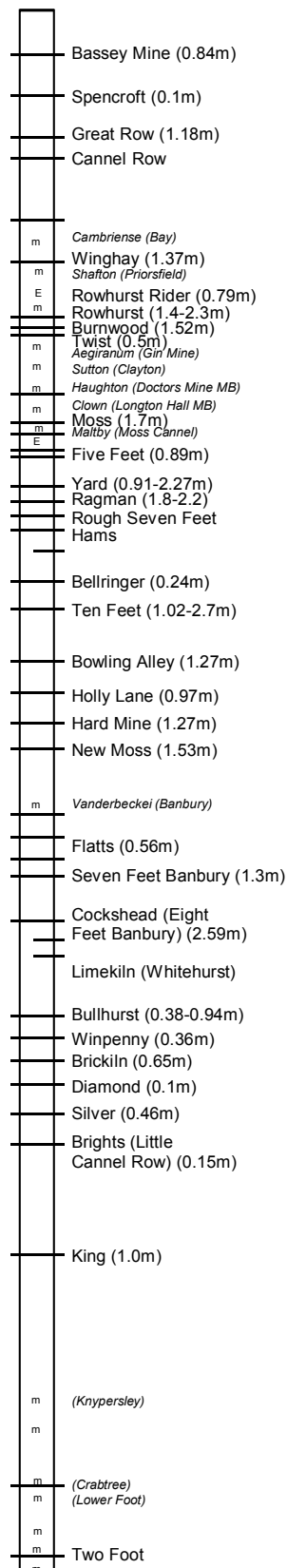
Figure 27. Stratigraphy of the main coal-bearing stratigraphic succession in the North Staffordshire Coalfield. Main seam names and thicknesses, where known, are labelled. m=marine band; E=Estheria band. Italicised text represent marine (or Estheria) band names.
