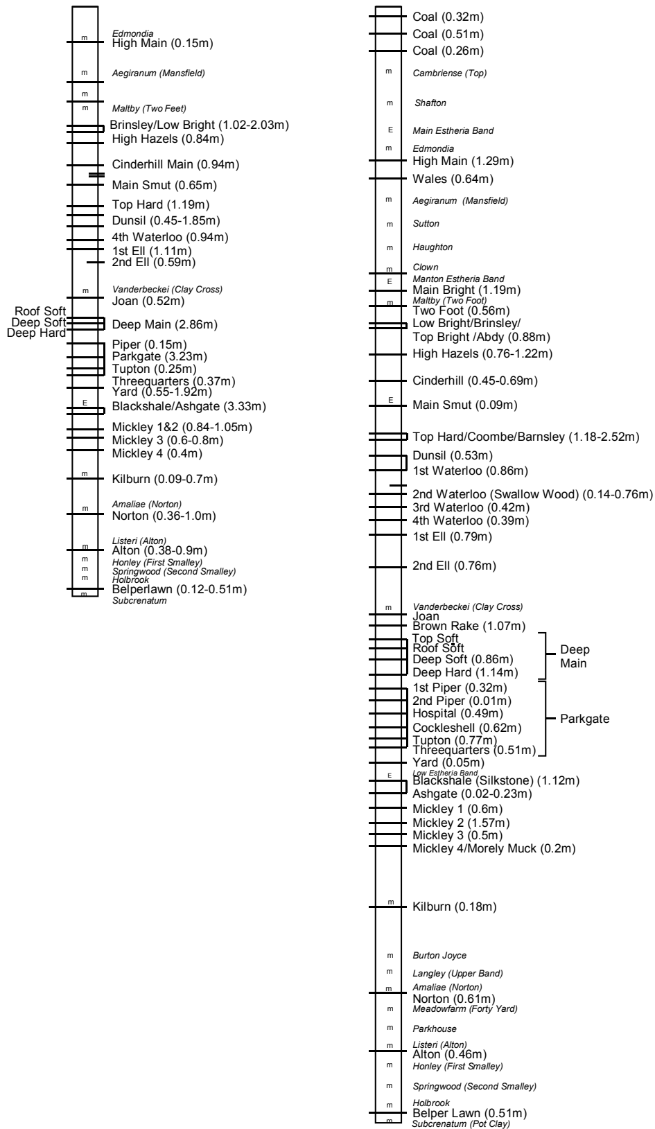
Figure 29. Stratigraphy of the main coal-bearing stratigraphic succession in the Nottinghamshire Coalfield. Main seam names and thicknesses, where known, are labelled. m=marine band; E=Estheria band. Italicised text represent marine (or Estheria) band names.
