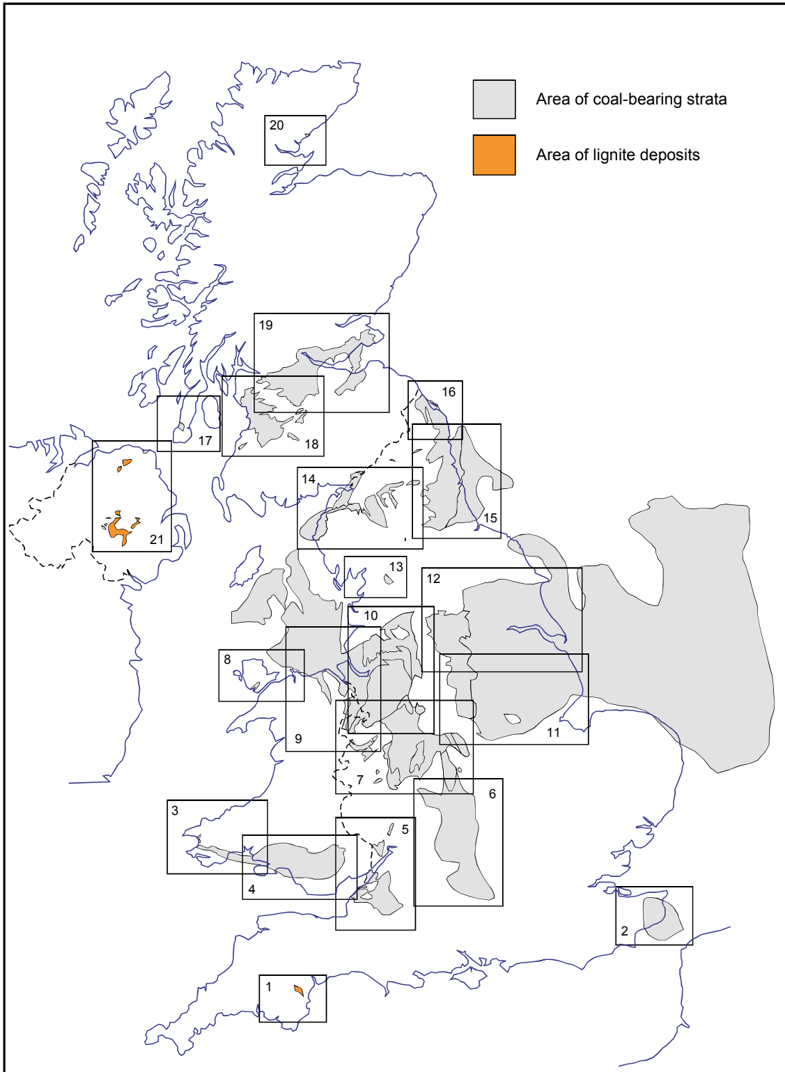
Figure 5. Map to show locations of the 1:100,000 scale mining and new technology maps produced by this study.
