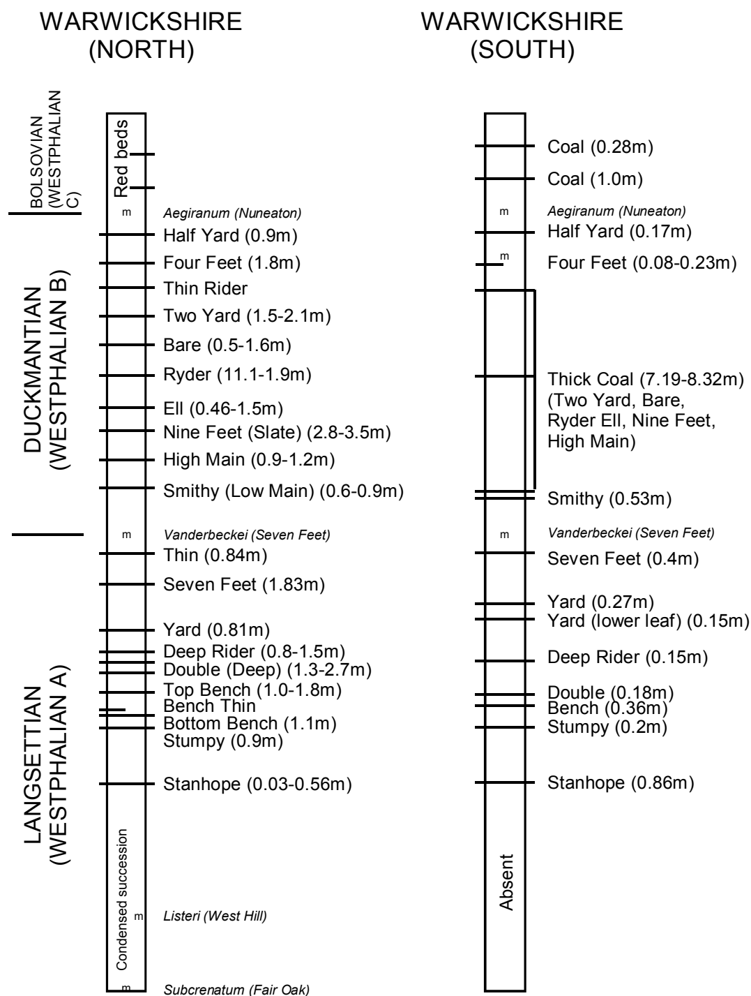
Figure 20. Stratigraphy of the main coal-bearing stratigraphic succession in the Warwickshire area. Main seam names and thicknesses, where known, are labelled. m=marine band; E=Estheria band. Italicised text represent marine (or Estheria) band names.
