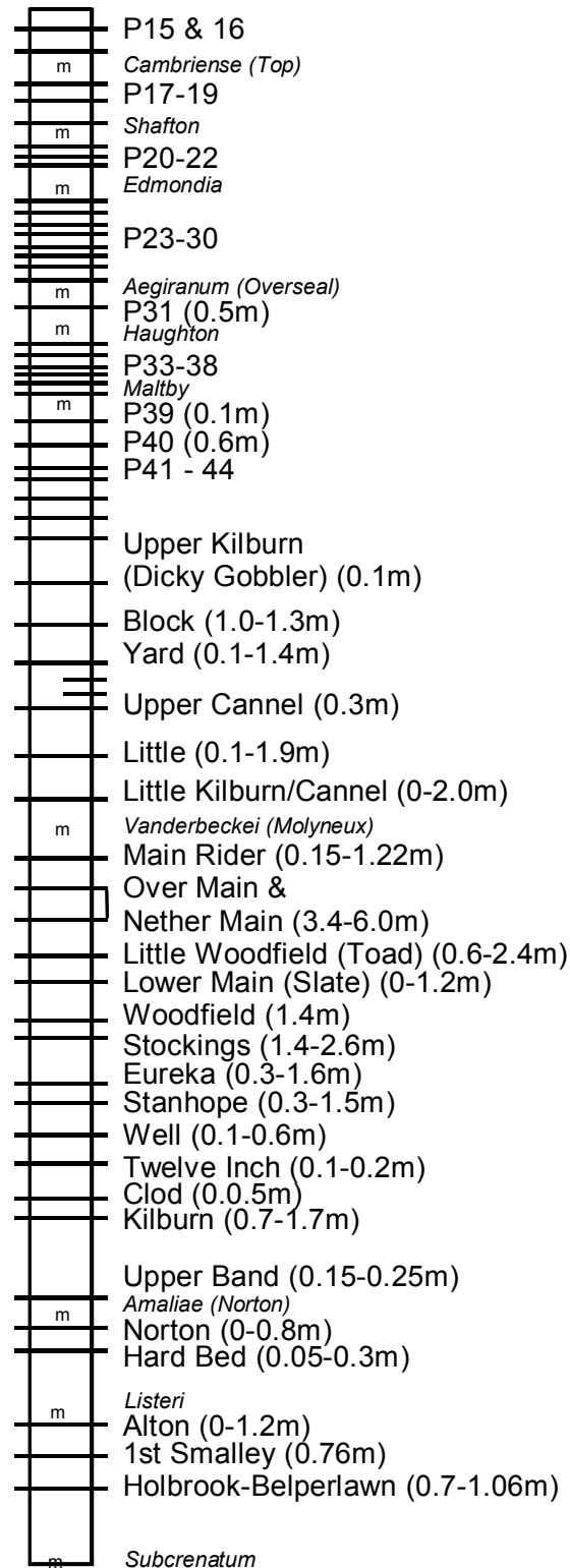
Figure 21. Stratigraphy of the main coal-bearing stratigraphic succession in the South Derbyshire Coalfield. Main seam names and thicknesses, where known, are labelled. m=marine band; E=Estheria band. Italicised text represent marine (or Estheria) band names.
