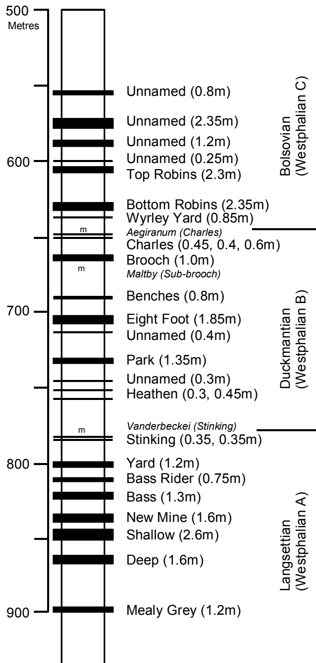
Figure 19. Stratigraphy of the main coal-bearing stratigraphic succession in the East Staffordshire area. Main seam names and thicknesses, where known, are labelled. m=marine band; E=Estheria band. Italicised text represent marine (or Estheria) band names.
