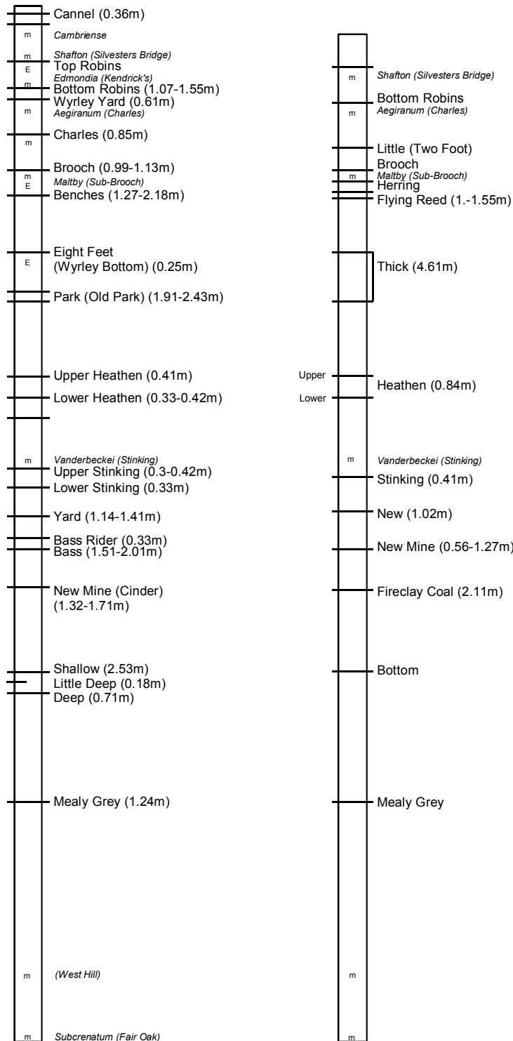
Figure 18. Stratigraphy of the main coal-bearing stratigraphic succession in the South Staffordshire Coalfield and Park Prospect area. Main seam names and thicknesses, where known, are labelled. m=marine band; E=Estheria band. Italicised text represent marine (or Estheria) band names.
