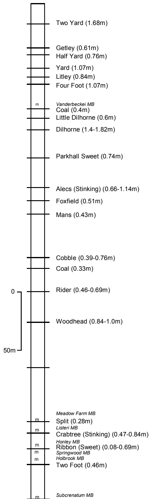
Figure 28. Stratigraphy of the main coal-bearing stratigraphic succession in the Cheadle Coalfield. Main seam names and thicknesses, where known, are labelled. m=marine band; E=Estheria band. Italicised text represent marine (or Estheria) band names.
